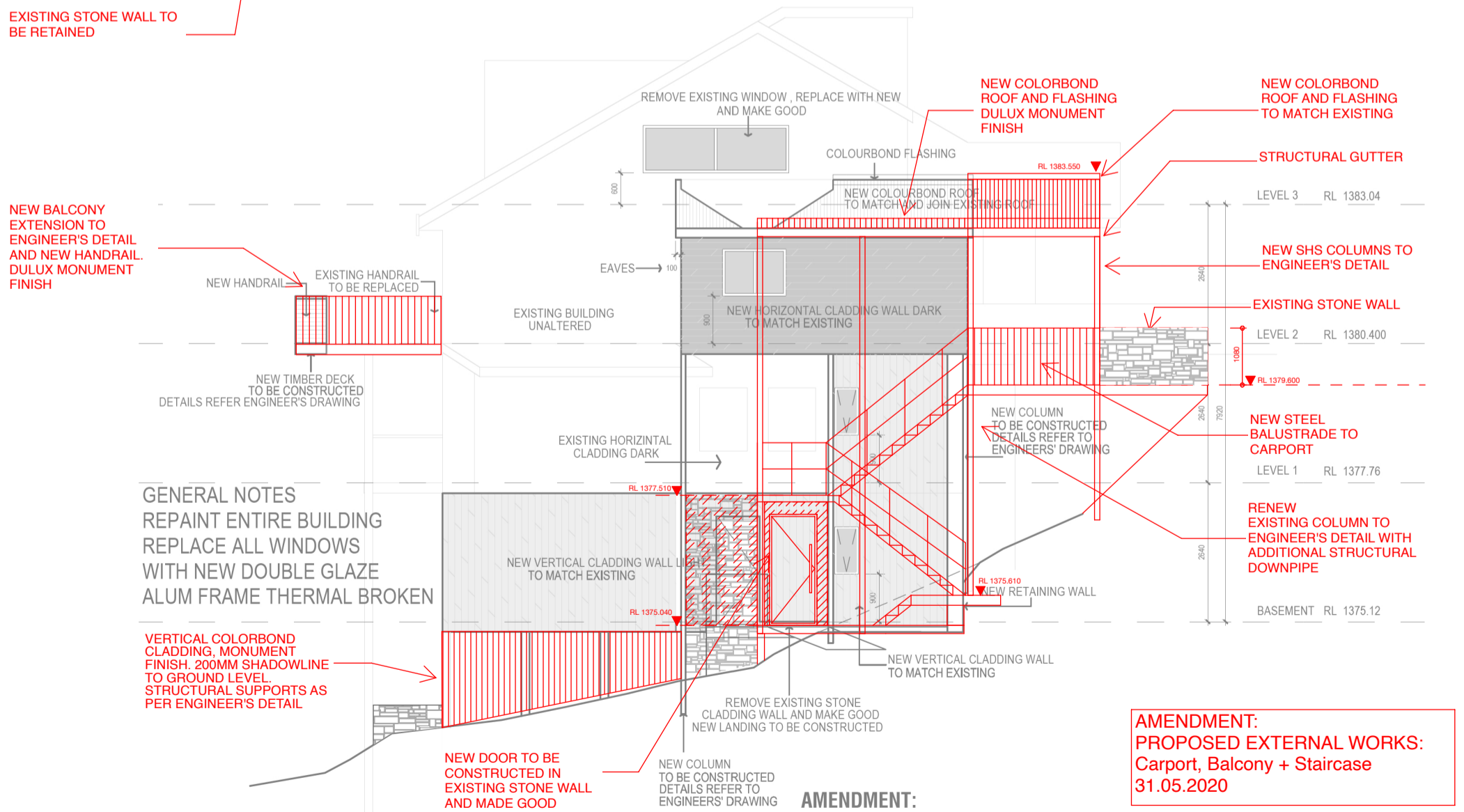
03 WEST ELEVATION SCALE 1:100 @ A3
